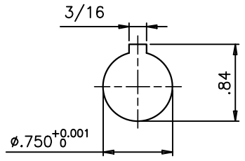
BORE KEYWAY
