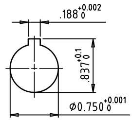
ROTOR BORE KEYWAY
